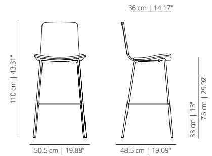
KLTFBAR_C lacquered with cushion
