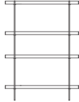
028-2502 Humla 100 tall shelf W1000 x D3450 x H1350
