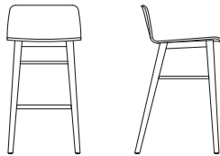
501-1302 Tami counter chair W430 x D505 x H865(SH665)
