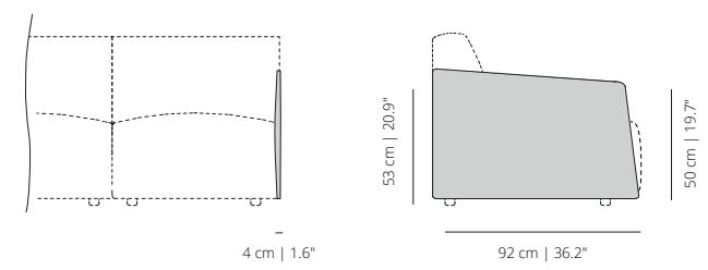
SISBRMEC medium backrest module
