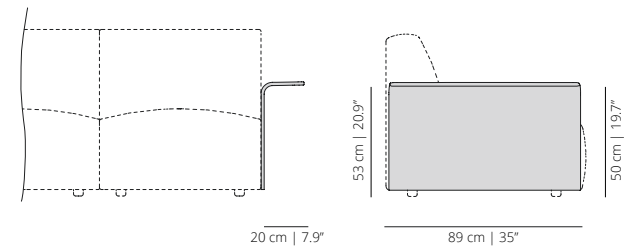
SISBRM curved wooden and/or upholstered arm
