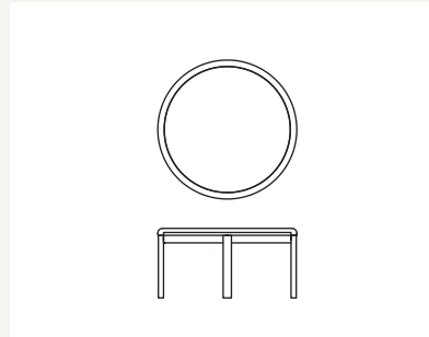
112-2103 Meld 72 Dia. 72 x H360
