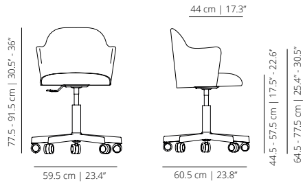
Caster base chair with arms
