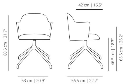
Pyramid swivel chair with arms
