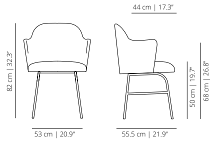
Metal base chair with arms
