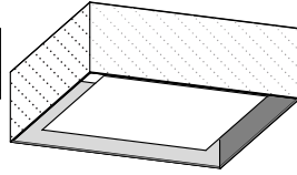
EXTERNAL & INTERNAL MATERIAL (RECOMMENDED WHEN DIFFUSER IS NOT FULL FIT)
