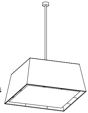
ROD SUSPENSION (OPTIONAL SWIVEL FOR RAKED CEILINGS)
