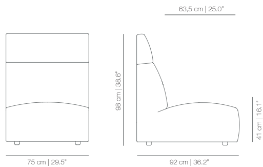
SISA - HIGH BACK MODULE
