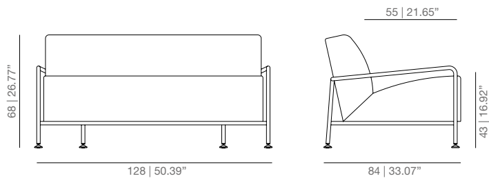
TA08 armchair 2 seats
